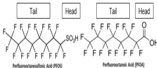
structure of PFAS compounds
